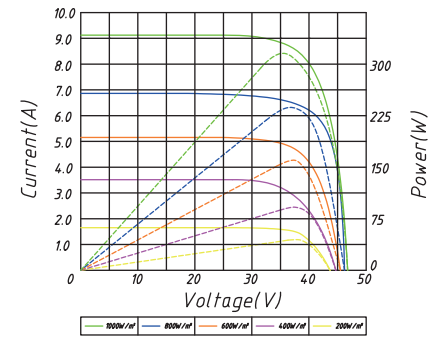
TP672P(H) Pm(W)310
