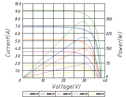
TP660P Pm(W)260
